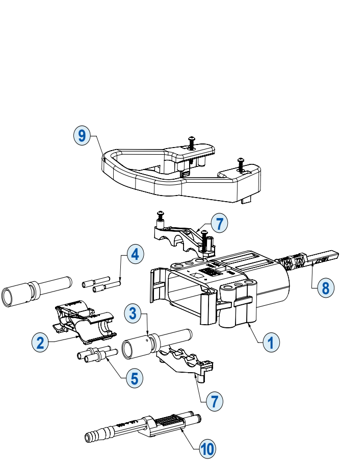
Male Connector
