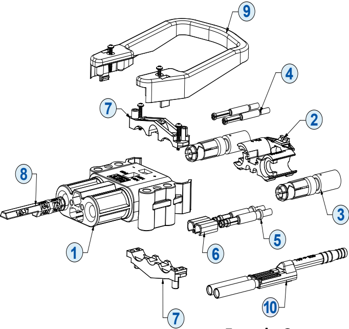
Female Connector
